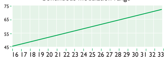
Consumption curve [NM 3 /h to kW el ]
