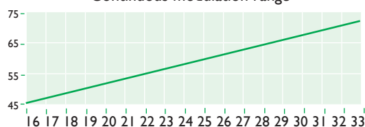
Consumption curve [NM 3 /h to kW el ]
